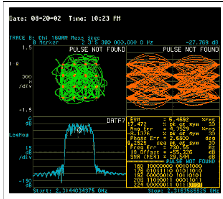
Figure 2. MAX2363 EVM at Pout = +5.3dBm
